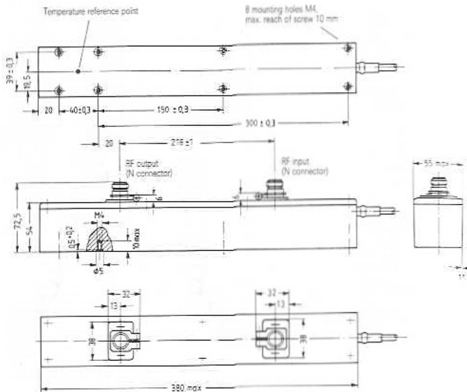
Outline drawing RW 248
