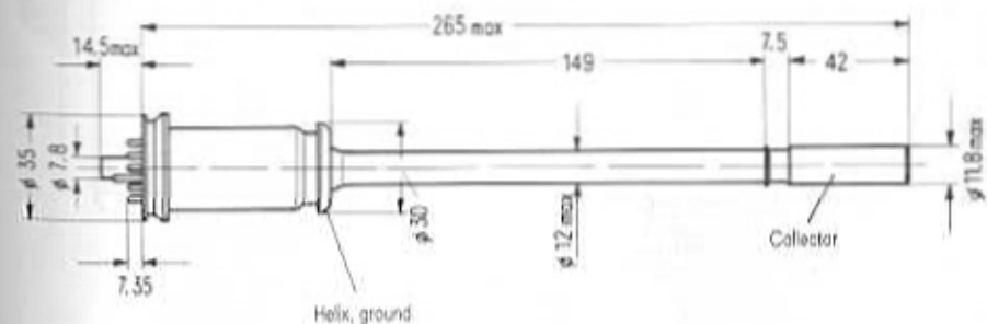
Traveling wave tube RW 81
