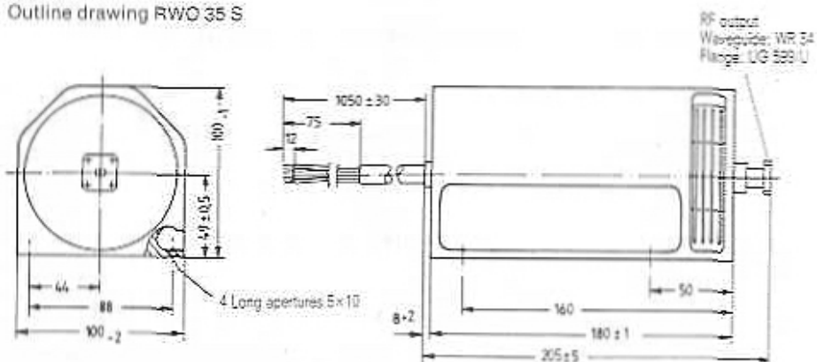
Outline drawing RWO 35 S
