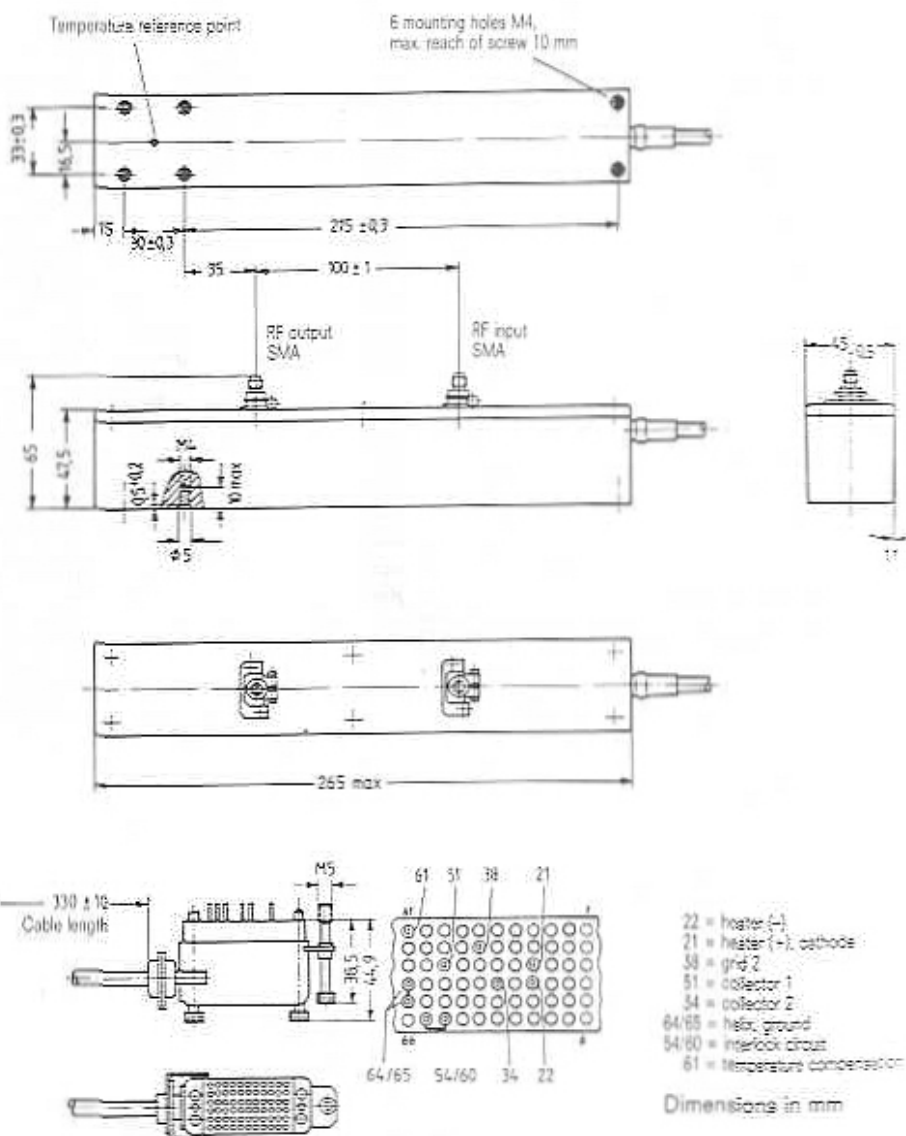
Outline drawing RW 1127
