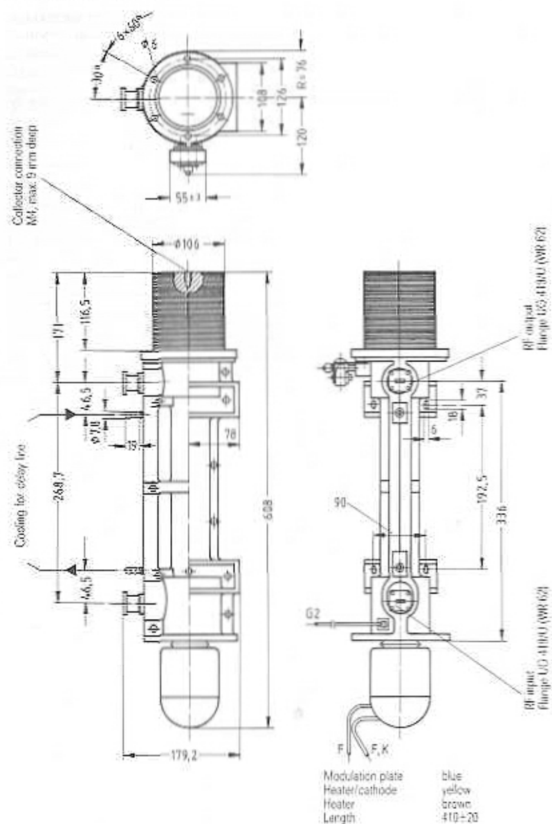
Outline drawing YH 1420
