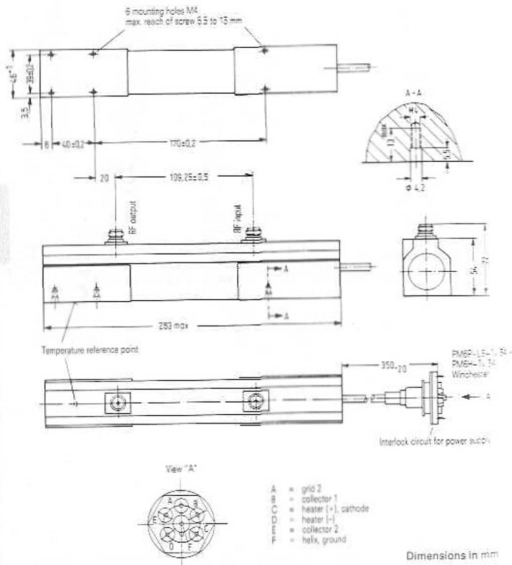
Outline drawing RW 88 C
