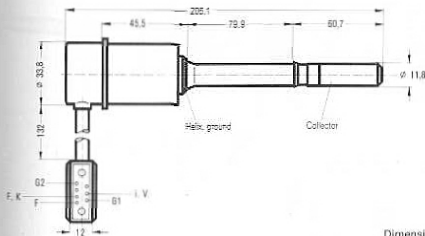
Traveling wave tube RW 70
