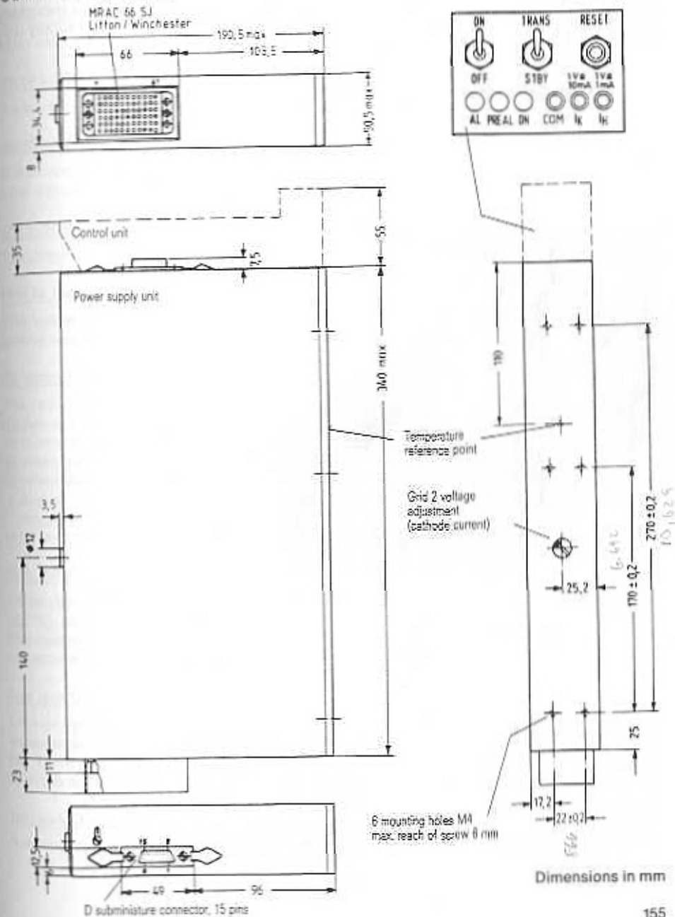
Outline drawing RWN 321
