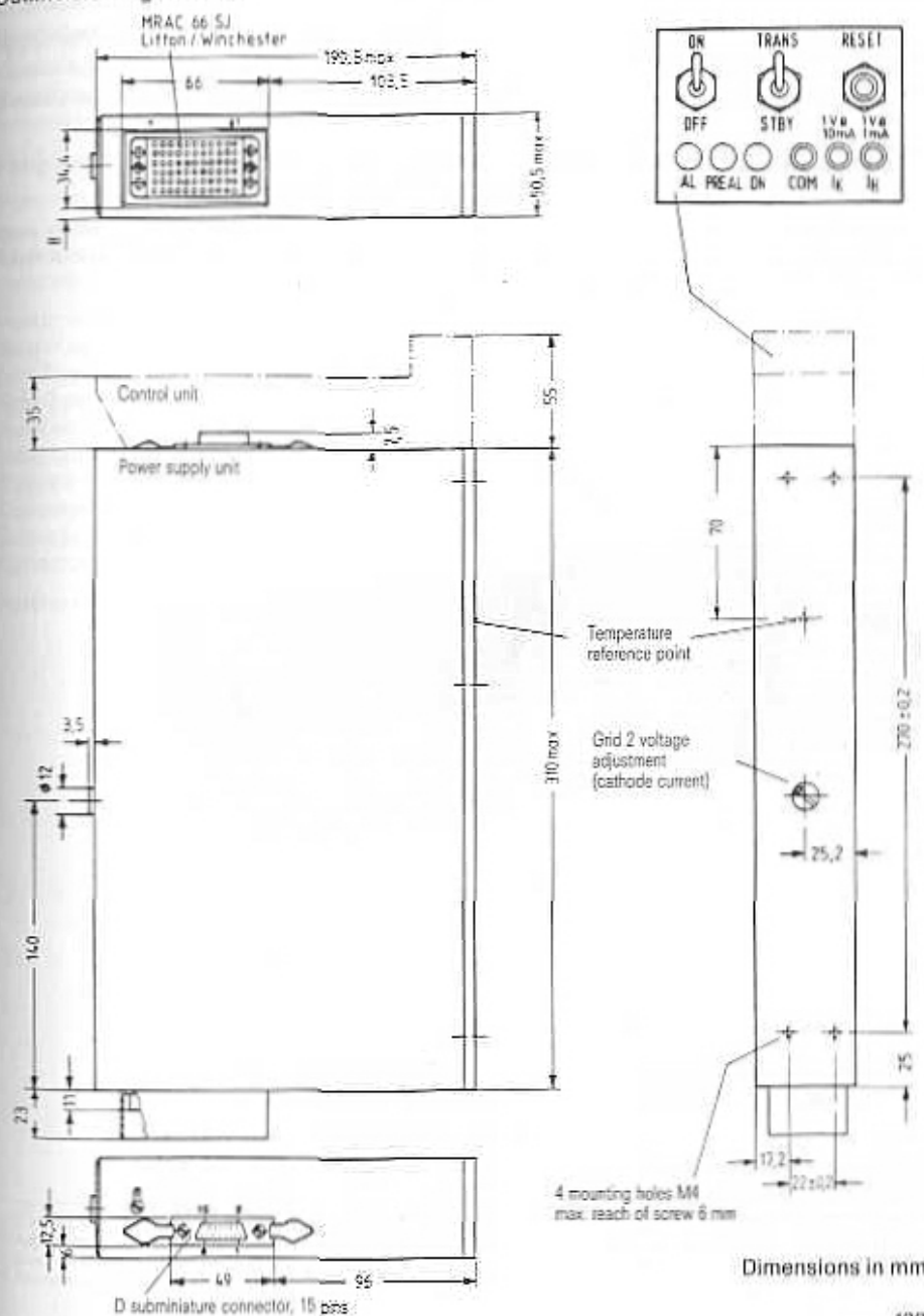
Outline drawing RWN 121
