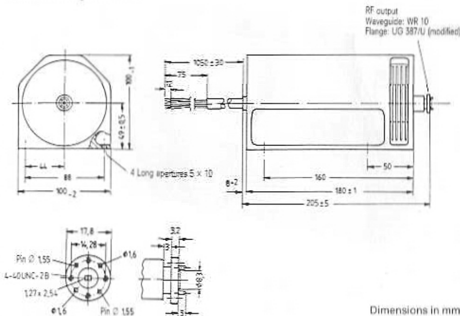
Outline drawing RWO 110 S
