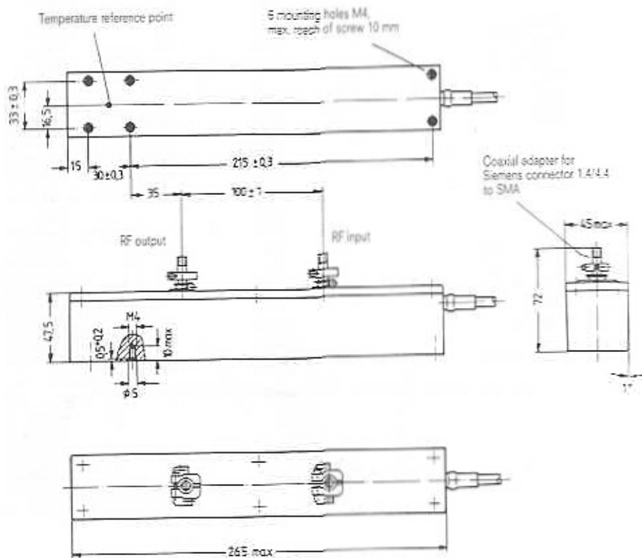
Outline drawing RW 1125 D
