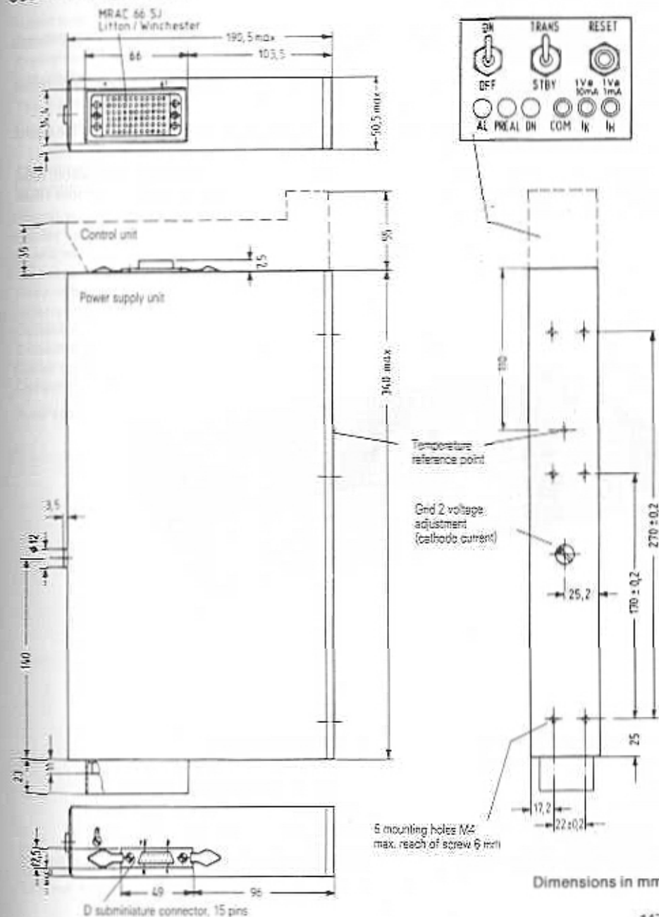
Outline drawing RWN 221
