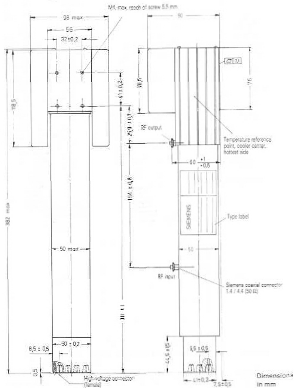
Outline drawing RW 85
