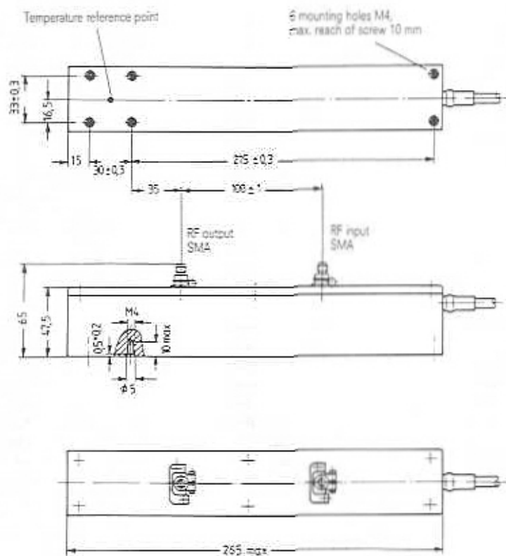
Outline drawing RW 1136
