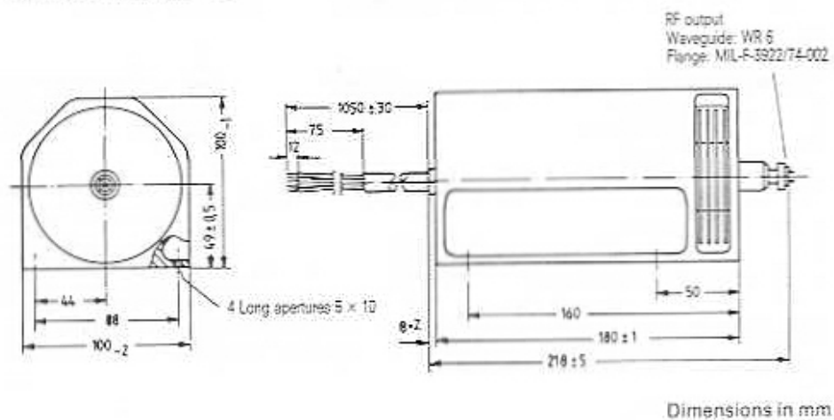
Outline drawing RWO 170
