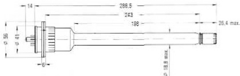
Traveling wave tube RW 3
