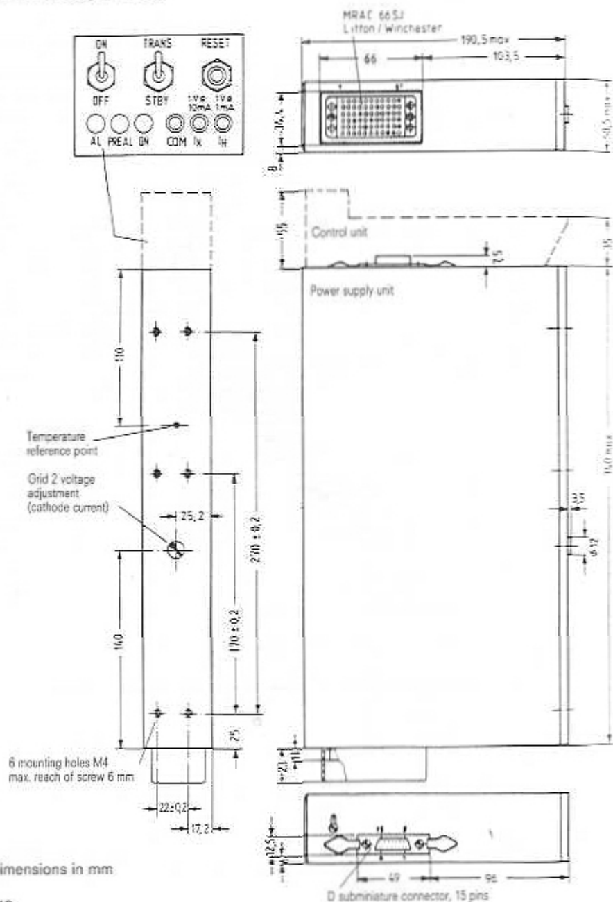
Outline drawing RWN 220
